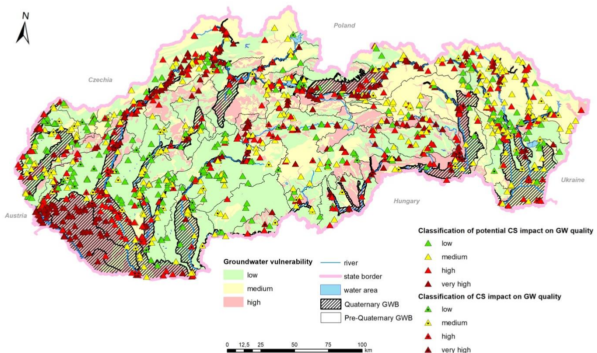
Fig. 1 Potential impact of contaminated sites (CS) on groundwater (GW) quality in Slovakia (classification from November 2020) GWB – groundwater body
